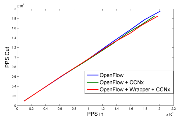
Fig. 2: Wrapper's impact on forwarding performance
